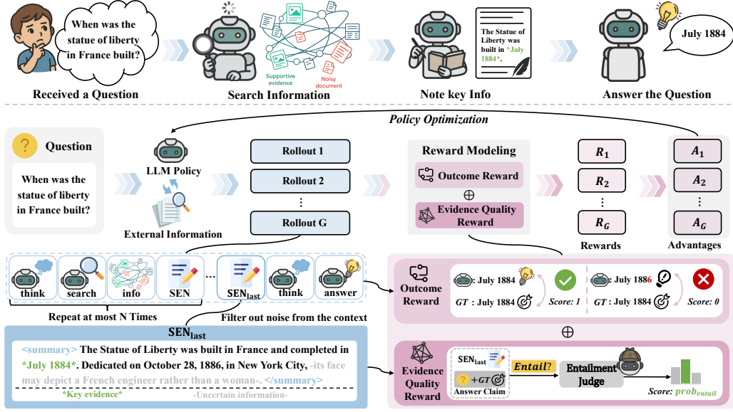
Figure 2: Overview of EviNoteRAG . To enhance RAG through quality-augmented evidence notes, the model is trained to generate Supportive-Evidence Notes (SENs) that retain only answer-critical information. An entailment-based Evidence Quality Reward (EQR) further ensures that each note faithfully supports the final answer, guiding the model toward more accurate and evidence-grounded reasoning.
