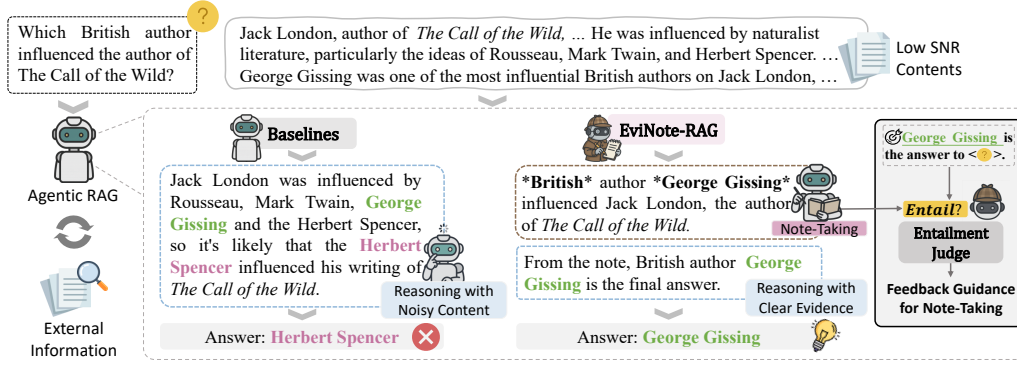
Figure 1: EviNoteRAG vs. Baselines (Song et al., 2025b; Jin et al., 2025): EviNoteRAG distills key information through evidence notes and, guided by an Entailment Judge, ensures that retained content directly supports the answer, thereby mitigating noise and enhancing performance.
