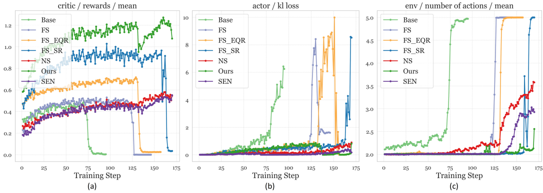
Figure 6: Training stability. Actor-side stability diagnostics across methods (Base, FS, FS+SR, FS+EQR, NS, SEN, and Ours = SEN+EQR). Panels: (a) reward score, (b) actor KL loss w.r.t. the reference policy. Lower and smoother curves indicate more stable optimization. (c) number of actions. When the model generates invalid actions, it tends to repeat the previous behavior, leading to a rapid increase in action frequency.
