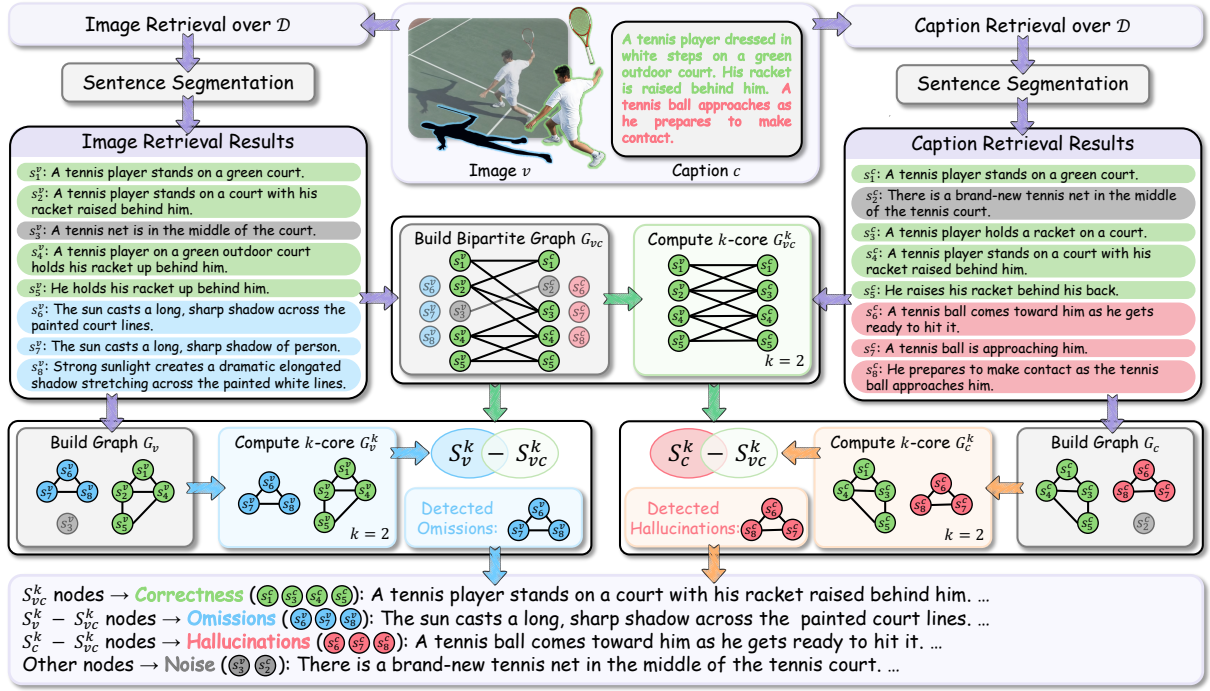
Figure 1: Reasoning strategy of Caption Refinement Suggester (CRS) and Caption Quality Assessor (CQA). We leverage k-core subgraph computation to analyze critical textual content in the retrieval results. Specifically, CRS extracts overlapping sentences S_v^k from the image retrieval results and uses them as signals to guide LVLMs to incorporate these key elements into their generated descriptions. By analyzing the discrepancy between S_v^k and caption-retrieved results S_c^k , CQA identifies hallucinations ( S_c^k - S_v^k ) and omissions ( S_v^k - S_v^c ) in this caption.
