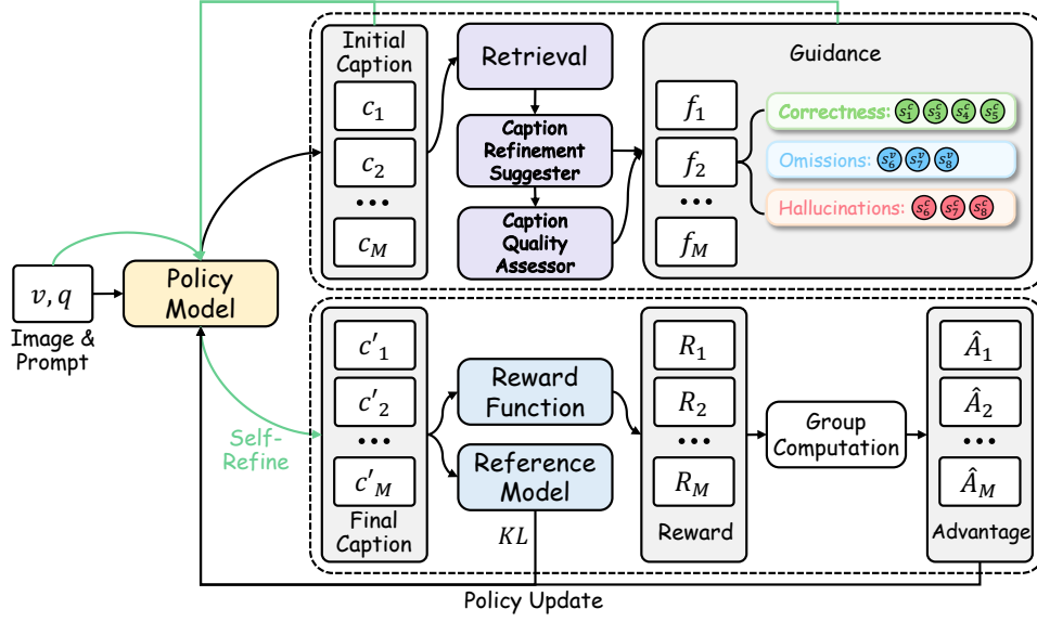
Figure 2: Overview of Retrieval-Guided Refinement for Image Captioning (Re 3 Cap) . Re 3 Cap begins by sampling initial captions \{c_i\}_{i=1}^M for each image v . Next, it performs image-conditioned retrieval and caption-conditioned retrieval, and leverages k-core analysis to generate guidance \{f_i\}_{i=1}^M based on Caption Refinement Suggester and Caption Quality Assessor. Finally, the method incorporates the guidance into prompts to obtain refined captions \{c'_i\}_{i=1}^M and optimizes the policy model with reinforcement learning.
