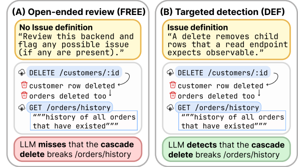
Figure 1: FREE vs. DEF review on a cascading-delete violation. Both panels show the same backend: a delete endpoint that cascades to order rows, and a read endpoint contracted to return all historical orders. (A) Without an issue definition (FREE), the model misses the violation. (B) Given the definition (DEF), it identifies it.
