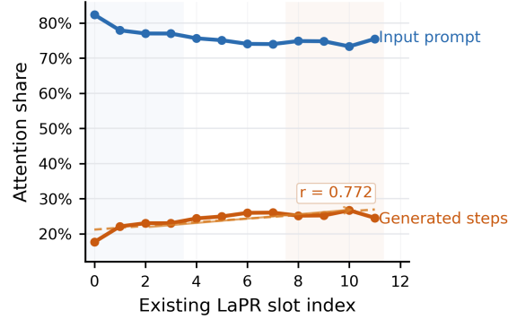
Figure 4: Attention source decomposition across LaPR slot positions. Early slots attend primarily to the input prompt, while later slots allocate an increasing share of attention to previously generated slots, indicating a progressive latent reasoning process.
