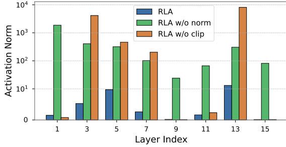
(a) L2 norm of attention output
