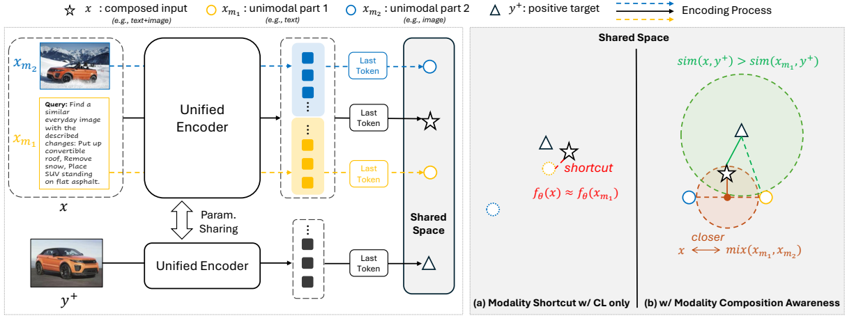
Figure 2: Modality Composition Awareness (MCA, §3.2). Unimodal parts are shown as dotted circles when not explicitly produced. (a) Training with vanilla CL: the composed embedding can be close to the target but still align disproportionately with one unimodal part, leading to modality shortcuts. (b) Training with CL and MCA: the composed embedding is explicitly constrained to be closer to the target than any of its unimodal parts by MCP (§3.2.1), and anchored to a compositional prototype mixed (Equation 5) from unimodal embeddings by MCR (§3.2.2) to mitigate modality shortcut.
