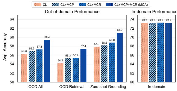
Figure 3: Breakdown of MCA through loss ablation.
