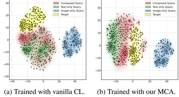
Figure 7: Visualizations of queries and targets.
