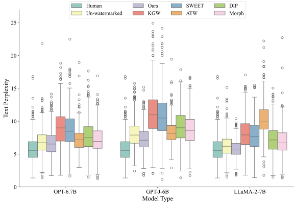
Figure 2: Comparison of text perplexity among human-written text, un-watermarked text, and texts using various watermarking methods conducted on different LLMs for C4 dataset.
