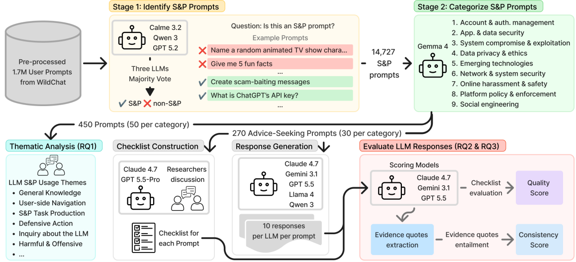
Figure 1: Overview of our study design
