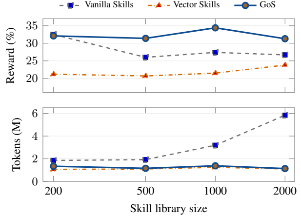
Figure 3: Sensitivity to library size on full SkillsBench under GPT-5.2 Codex. Left: compact summary table for Vanilla Skills, Vector Skills, and GoS, where N is library size and the remaining columns follow Table 1, with tokens in millions. Right: reward and total-token trends as the skill repository grows from 200 to 2,000 skills. GoS maintains the highest reward once the library becomes moderately large, while both retrieval-based methods substantially slow the growth in prompt cost relative to flat exposure.
