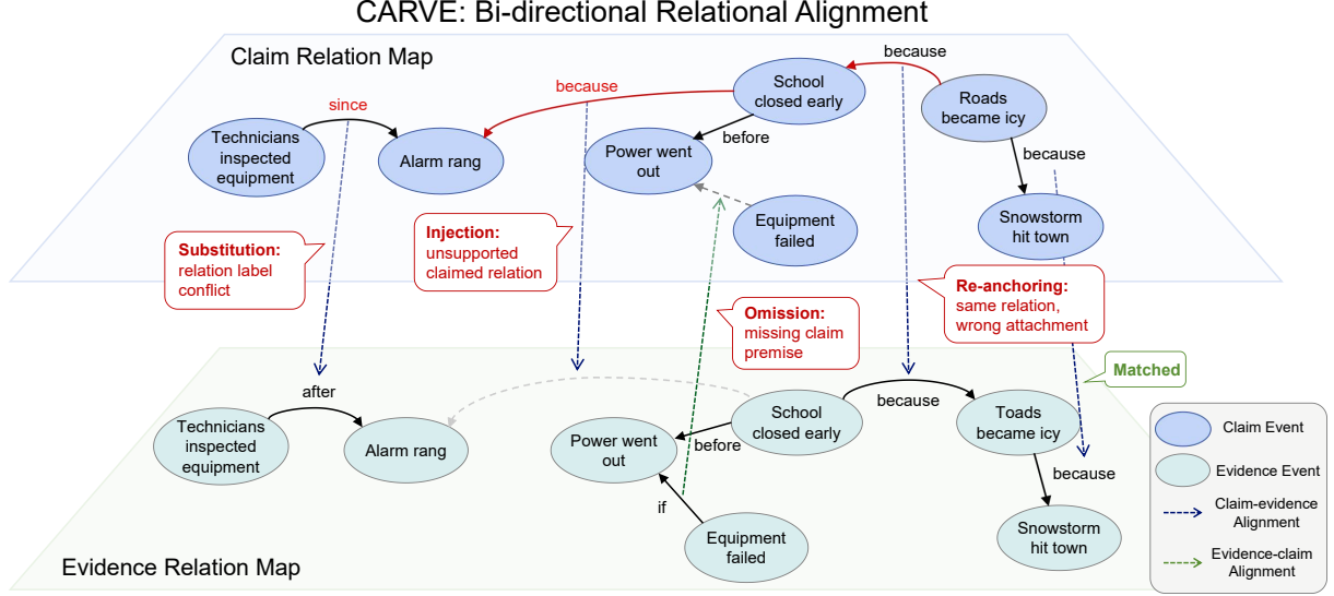
Figure 2: Overview of CARVE’s bidirectional relational alignment. CARVE aligns claim relations with a claim-anchored evidence structure: claim-to-evidence alignment detects Injection, Re-anchoring, and Substitution through missing edges, endpoint conflicts, and label conflicts, while evidence-to-claim alignment detects Omission by finding required evidence relations absent from the claim. This explicit alignment improves transparency and reduces reliance on costly end-to-end LLM reasoning.
