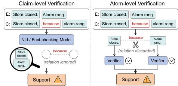
Figure 1: Limitation of current paradigms on relationally corrupted claims. Claim-level verifiers misclassify due to entity-overlap bias. Atom-level decomposition systematically discards logical connections.
