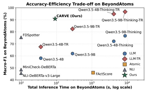
Figure 3: Inference efficiency comparison on BEYONDATOMS. The x-axis uses a log scale due to the large runtime gap across models.
