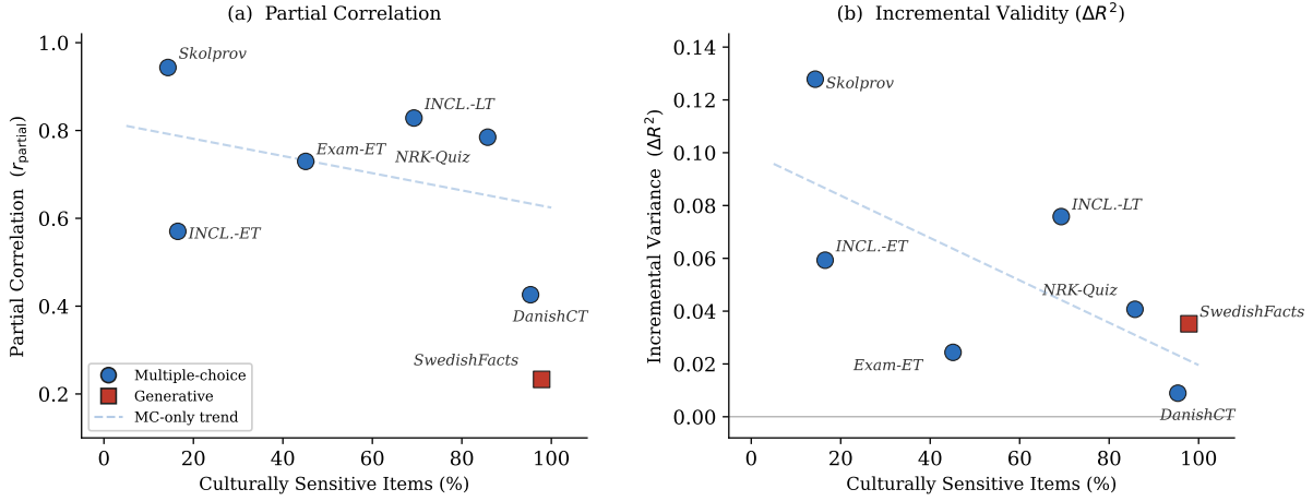
Figure 1: Proxy validity as a function of cultural sensitivity. Each point represents one native-vs-proxy pairing. (a) Partial correlation after residualizing on controls. (b) Incremental variance ( \Delta R^2 ) from the nested F -test. The dashed line shows the MC-only linear trend (6 pairings; descriptive and not statistically significant at n = 6 ). DanishCitizenTest (95% CS, MC format) already shows weak incremental validity. SwedishFacts lies close to the descriptive MC extrapolation in panel (b), which is consistent with a locality/content-overlap interpretation, but the design does not isolate locality from its open-ended response format.
