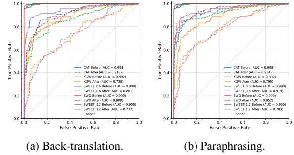
Figure 5: Watermark detection performance against two attacks. We set \gamma = 0.5 and \delta = 2.0 for watermark methods and \rho = 5, \alpha = -2 for CATMARK.
