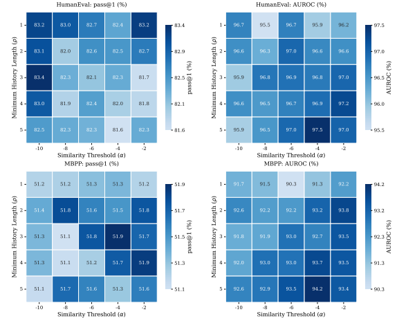
Figure 3: Detailed pass@1 and AUROC of CATMARK across \alpha and \rho , with \gamma = 0.5 and \delta = 2.0 fixed.
