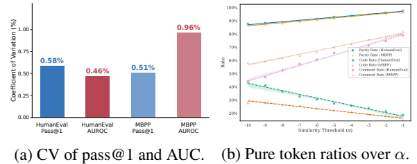
(a) CV of pass@1 and AUC. (b) Pure token ratios over \alpha .
