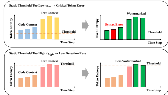
Figure 1: Illustration of the "Trade-off Dilemma" with static entropy thresholds in cross-task generation. A fixed low threshold compromises the functional correctness of structured data like code (Top), while a fixed high threshold significantly diminishes watermark detectability in natural language text (Bottom).
