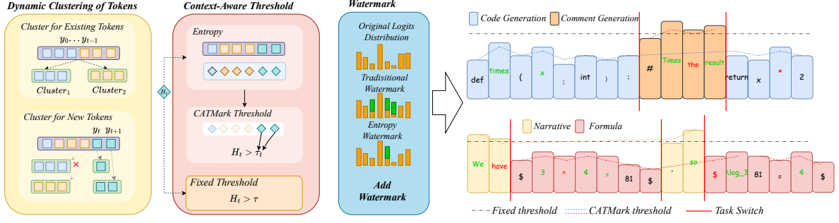
Figure 2: Comparison between static-threshold watermarking and our context-aware, cluster-based thresholding method, CATMARK. Our approach dynamically clusters generated tokens based on logit similarity (left panel), then computes a context-specific entropy threshold per cluster using historical entropy sequences (middle panel). Tokens whose entropy exceeds the adaptive threshold are watermarked (right panel). In the token sequence visualizations, rectangle height represents normalized entropy.
