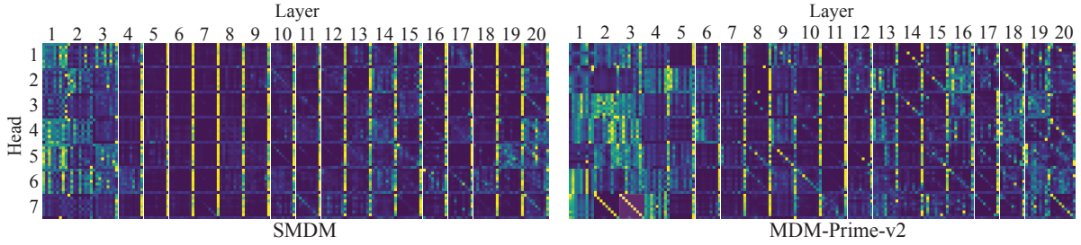
Figure 9: Attention score patterns of SMDM and MDM-Prime-v2. Both models contain 20 layers and 14 attention heads. A complete plot of all heads is shown in Fig. A7. MDM exhibits vertical stripes across Layers 4–20. In contrast, MDM-Prime-v2 displays diagonal structures and a richer diversity of patterns.
