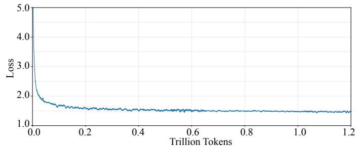
Figure A9: Training loss curve of MDM-Prime-v2 (7B) over the course of pre-training. The model is trained on 1.2T tokens using the Dolma-6T dataset.
