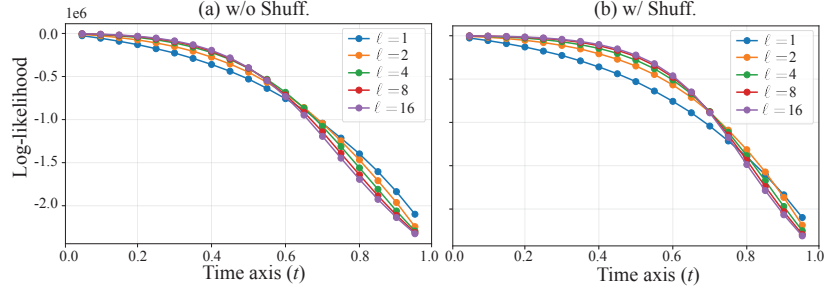
Figure A5: Log-likelihood of MDM ( \ell = 1 ) and MDM-Prime ( \ell > 1 ) across time. Subplots (a) and (b) show the results without and with the index shuffling operation, respectively. The maximum value for each curve is 0.
