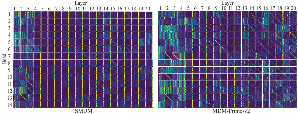
Figure A7: Attention score patterns of SMDM and MDM-Prime-v2. Both models adopt the same model architecture containing 20 layers and 14 attention heads. SMDM exhibits vertical stripes across deeper layers (e.g., Layers 4–20). In contrast, MDM-Prime-v2 displays diagonal structures and a richer diversity of patterns.
