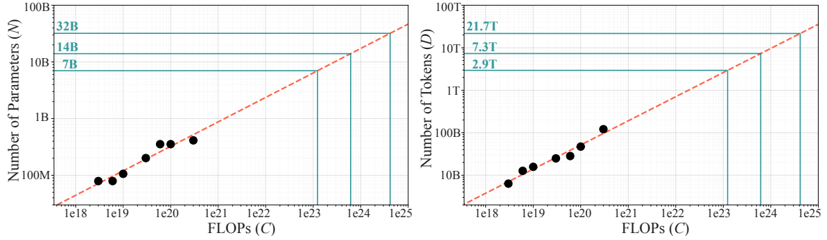
Figure A8: Compute-optimal allocation of the number of non-embedding parameters ( N ) and training tokens ( D ) for MDM-Prime-v2 under different FLOPs ( C ). Left: Optimal N as a function of C . Right: Optimal D as a function of C . Black points represent the compute-optimal empirical samples. The red dashed lines indicate the fitted power-law regression extended to larger budgets. Teal annotations highlight the training token counts required to optimally train models of specific target sizes (e.g., 7B, 14B, and 32B).
