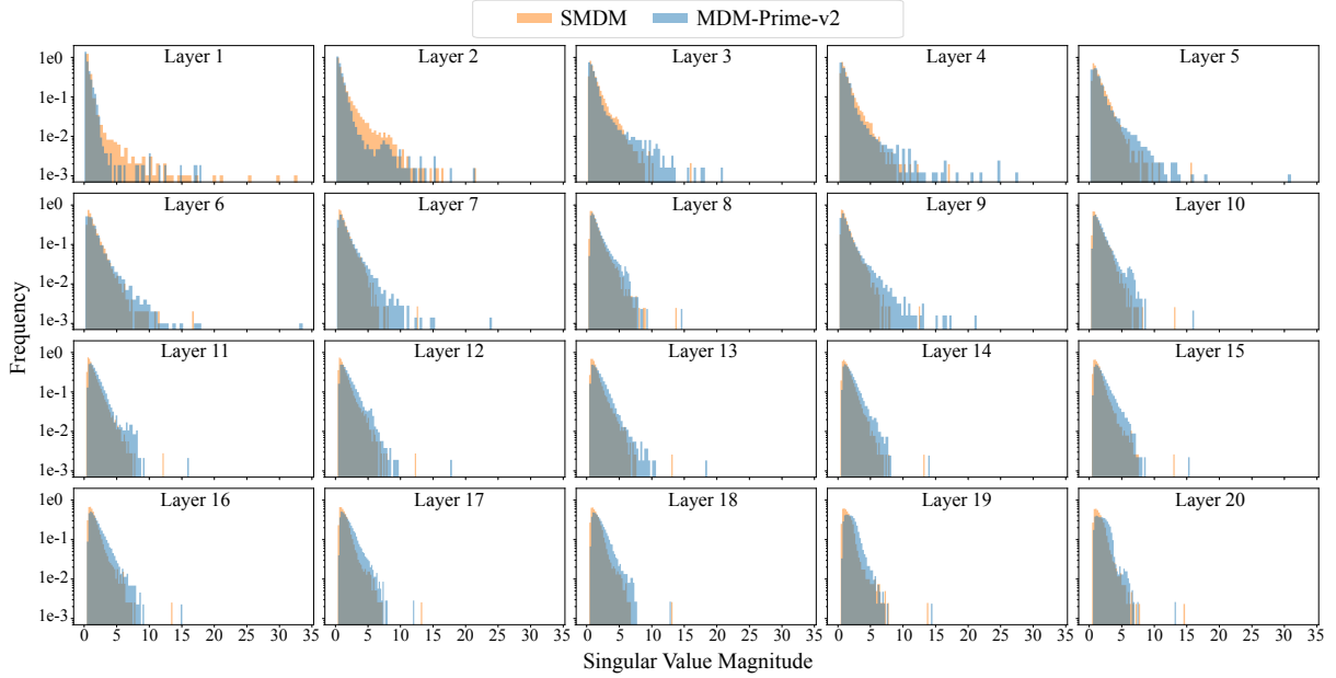
Figure A6: Singular value distributions of the query-key-value projection matrices of SMDM (1.1B) (Nie et al., 2025a) and MDM-Prime-v2 (1.1B). Both SMDM and MDM-Prime-v2 adopt the same architecture containing 20 layers. The y-axis represents frequency on a log scale. Compared to MDM, MDM-Prime-v2 exhibits a heavier-tailed distribution, particularly in intermediate layers (i.e., Layers 3–12).
