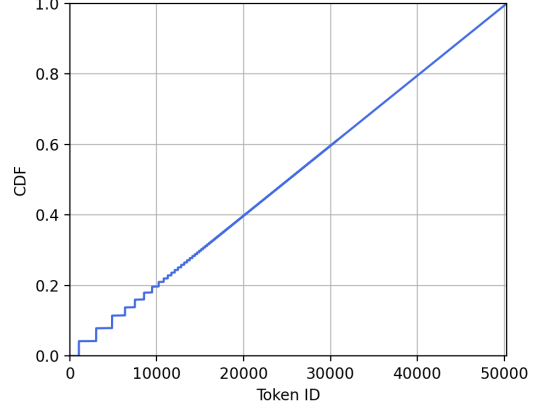
Figure A10: Cumulative distribution function (CDF) of token indices under greedy assignment, computed using the GPT-2 tokenizer on C4.
