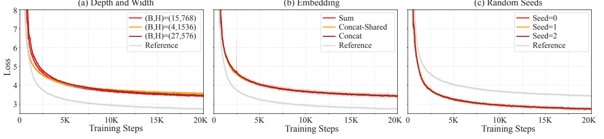
Figure A4: Analysis of performance invariance in MDM-Prime and MDM-Prime-v2. The plots show robustness against variations in: (a) model architecture depth and width; (b) embedding table designs; and (c) random seeds for the index shuffling operation.
