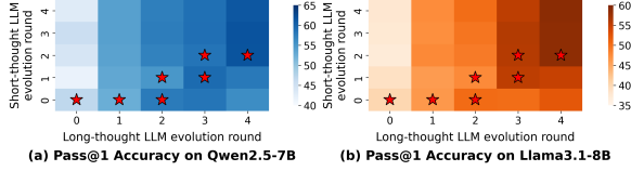
Figure 4: Pass@1 accuracy evolution during asynchronous policy updates. Red stars indicate selected model checkpoints.
