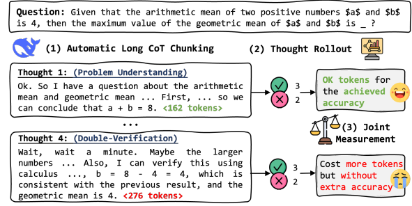
Figure 1: Thought importance analysis framework. Given a long CoT, we automatically chunk it into multiple thought blocks and perform Monte Carlo rollouts to evaluate how individual thoughts affect reasoning effectiveness and efficiency.
