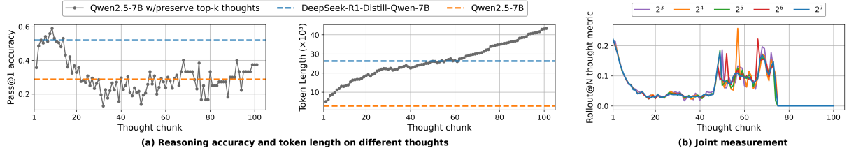
Figure 2: (a) How thoughts affect Pass@1 accuracy and token length on GPQA. We investigate how long thoughts from DeepSeek-R1-Distill-Qwen-7B affect the accuracy and token length of Qwen2.5-7B. The cyan line represents the effectiveness upper bound with full long thoughts; the orange line indicates the baseline under full short thoughts. (b) Joint measurement of thought effectiveness and efficiency as Monte Carlo rollout count increase from 2^3 times to 2^7 times.
