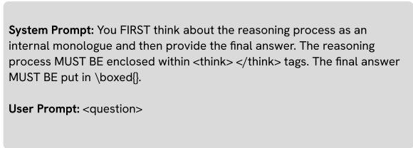
Figure 4: Example prompt used to distill reasoning traces from the ThinkLite model.
