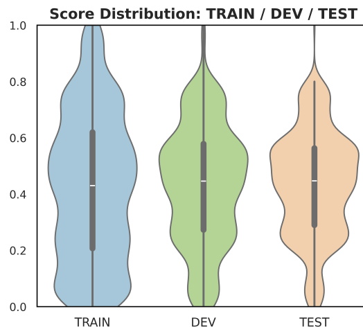
Figure 2: Score distributions for each split
