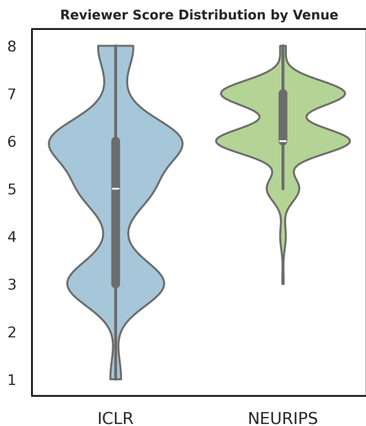
Figure 1: Reviewer rating distribution for ICLR and NeurIPS.
