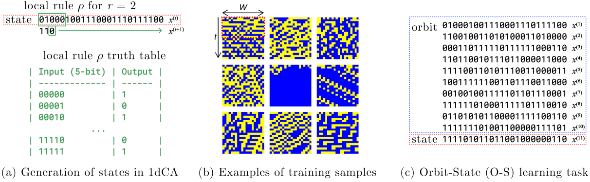
Figure 1: Learning One-dimensional Cellular Automata (1dCA). (a) Update of state with local rule. (b) Orbit of 1dCA is a sequence of binary strings of size W = 20 . The first k = 10 states marked by the red rectangle encode transformer input. (c) Given a part of the orbit a model learns to predict the next state (O-S).
