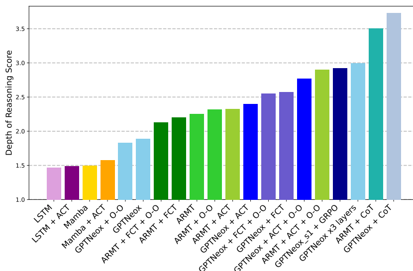
Figure 5: With GRPO as well as with ACT and Orbit-Orbit training depth of reasoning can be significantly extended. Average DepthScore = 1 + \sum_{k=2}^4 \text{exact\_match}(k) , where \text{exact\_match}(k) is the exact match accuracy of predicting the (10 + k) th state based on the first 10 states. Results also include FCT (Fixed Computation Time) ablation which is described in subsection J.1
