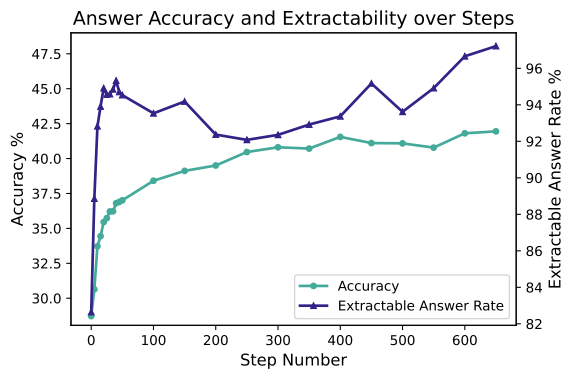
Figure 6: MMLU-Pro answer accuracy and extractability for 1.5B model on WildSci (Majority-Aligned). Accuracy continues to rise even as extractability stabilizes, indicating reasoning improvements beyond formatting effects.
