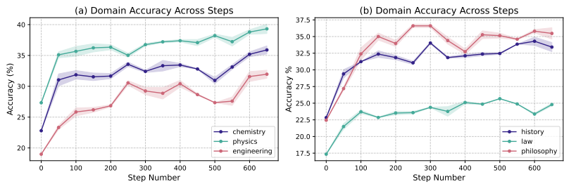
Figure 5: Domain-specific accuracy trends on MMLU-Pro during training. We report mean accuracy across three runs for each domain. Shaded regions indicate standard deviation. (a) shows steady improvements in domains with higher WildSci coverage (chemistry, physics, engineering), while (b) illustrates more variable performance in domains with lower coverage (law, history, philosophy).
