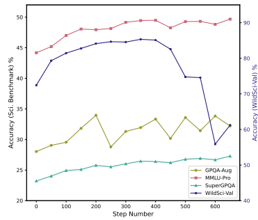
Figure 4: Performance trends on validation and test sets during training of the 3B model on WildSci All Aligned. The model exhibits continued generalization on test sets even after overfitting on the valid set.
