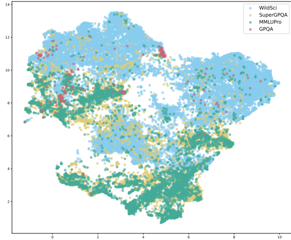
Figure 10: UMAP illustration.
