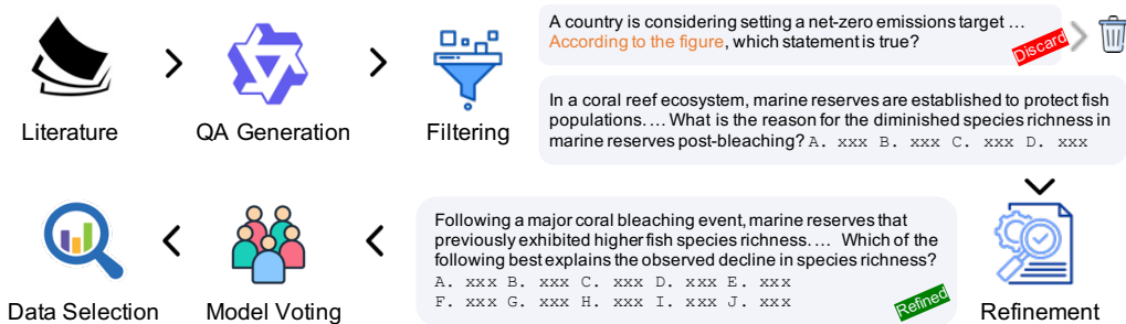
Figure 1: Overview of WildSci’s data creation pipeline. Filtering is based on heuristic rules, while refinement expands the option space and rephrases questions to increase diversity.
