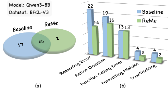
Figure 6: Statistics of failed tasks with and without ReMe. (a) Left: shows overlapping and unique failure cases; (b) Right: displays the number of task failures across different error categories.
