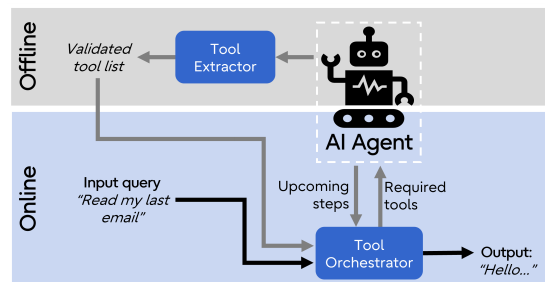
Figure 1: AGENTRIM Framework : An offline tool extractor reconstructs and validates the agent's tool inventory; an online tool orchestrator dynamically shapes per-step tool access while preserving the agent's logic.
