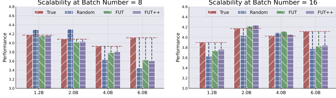
Figure 6: Scalable estimation performance across model sizes. We evaluate the estimation accuracy of FUT and FUT++ across model scales \{1.2\text{B}, 2.0\text{B}, 4.0\text{B}, 6.0\text{B}\} under training batch numbers T = 8 (left) and T = 16 (right). FUT and FUT++ consistently outperform the Random baseline, with FUT++ showing improved accuracy for larger models.
