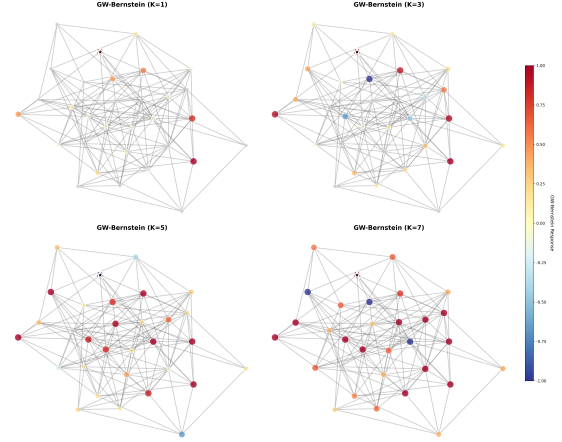
Figure 5: Spatial influence patterns learned by our multi-scale Bernstein-based graph filters.
