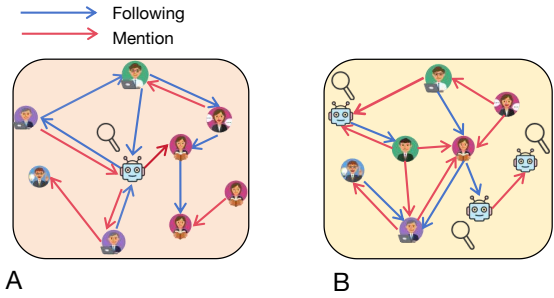
Figure 1: Illustration of social network bot detection and the concept of graph homophily. The task aims to distinguish bots from genuine users in complex social network. In Community A, high homophily is observed because most connections occur between nodes with the same labels, such as humans connecting to other humans. In Community B, low homophily or heterophily emerges due to interactions between nodes with different labels, specifically where bots connect to genuine users. Since these varying homophily levels result in distinct graph spectral features, model must adaptively focus on specific frequency bands to effectively capture bot-specific signals.
