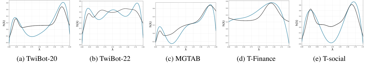
Figure 4: Learned spectral filter h(\lambda) for different datasets by HW-GNN (blue) and original Bernstein polynomial (black).
