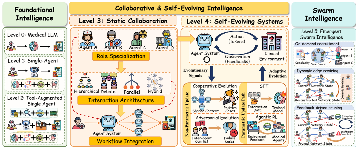
Figure 1: Overview of the proposed L0–L5 evolutionary taxonomy for MMAS.
