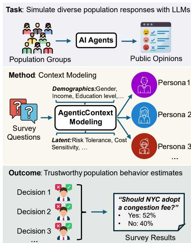
Figure 1: Conceptual overview of context modeling for population-level behavior simulation with LLMs.
