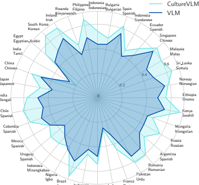
Figure 7: Results on CVQA (Romero et al., 2024).
