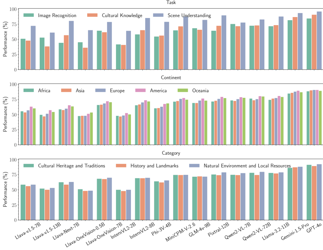
Figure 3: Different models on three tasks (upper), five regions (middle), and three categories of concepts (lower).
