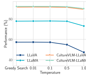
Figure 8: Impact of different decoding temperatures on performance.
