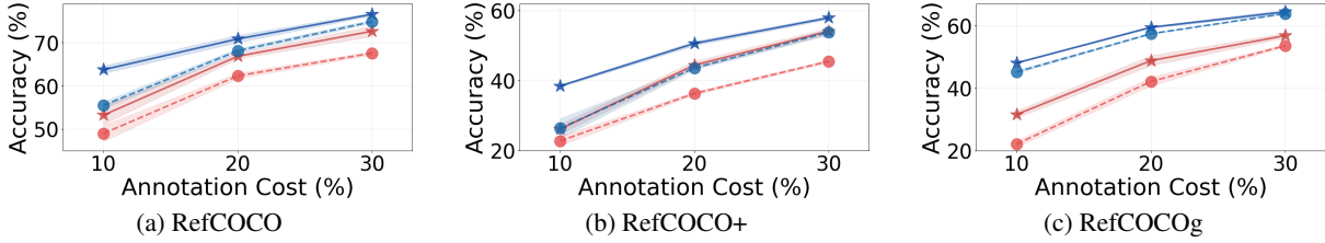
Figure 6: Comparison with the naïve labeling and random acquisition on a REC task. The reported results are averaged on the val and test (A,B) splits of each dataset. The annotation cost (x-axis) is calculated as the measured cost of the acquired samples via used labeling tool divided by the total manual annotation cost of the dataset.
