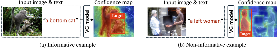
Figure 2: Illustration of informativeness in VG: (a) the model assigns high confidence to multiple regions, indicating an informative sample, while (b) a referred one is solely activated by the model, showing low informativeness.
