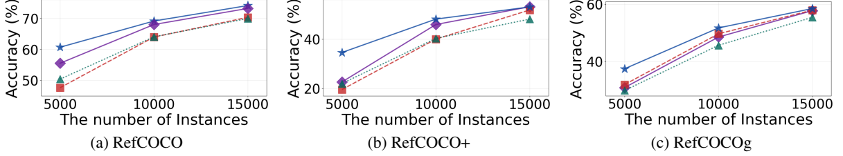
Figure 8: Comparisons with several acquisition baselines on a REC task. By comparing performance based on the number of acquired instance-text pairs, we isolate the effectiveness of each acquisition from the annotation tool.
