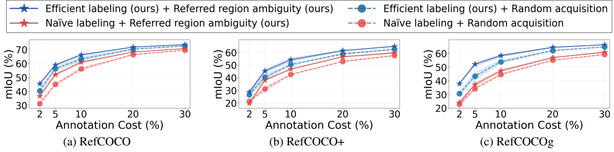
Figure 5: Comparison with the naïve labeling and random acquisition on a RIS task.
