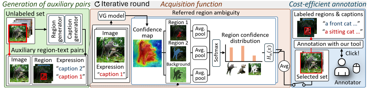
Figure 3: The proposed AL framework for visual grounding. We first generate auxiliary region-text pairs for all raw images in the entire unlabeled pool (Sec. 3.2). Following this, iterative rounds of sample selection and labeling begin. In each round, our referred region ambiguity (Sec. 3.3) scores the informativeness of all raw images by utilizing their auxiliary region-expression pairs. The top-scoring images are then sequentially annotated via our cost-efficient interface (Sec. 4) until the round budget is exhausted.
