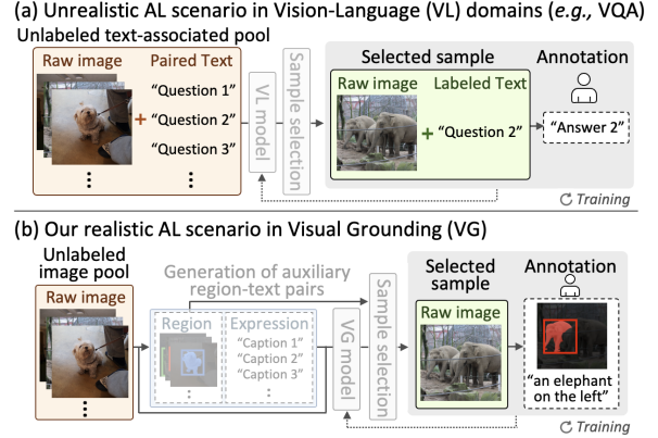
Figure 1: Illustration of AL settings in vision-language domains: (a) existing unrealistic scenario (Kim et al., 2021; Lin and Parikh, 2017) in VQA assumes that costly textual questions related to each image are already available in the unlabeled pool, whereas (b) our realistic setting in VG considers a practical scenario where only raw images are provided without textual descriptions.
