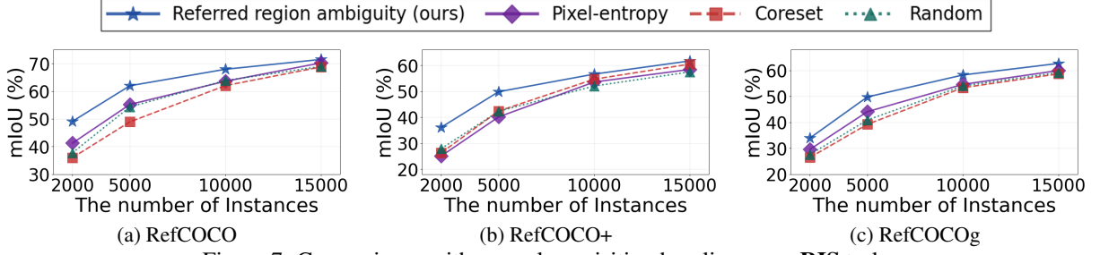
Figure 7: Comparisons with several acquisition baselines on a RIS task.
