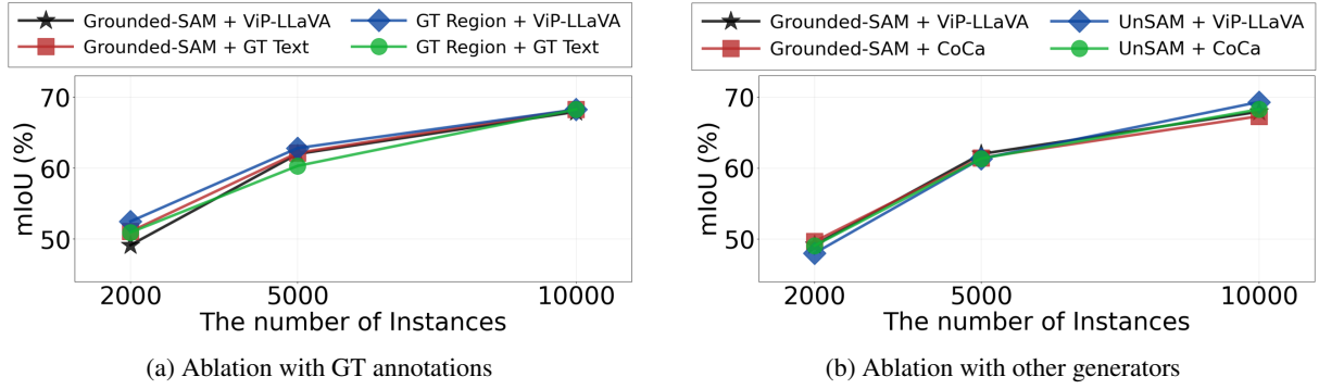
Figure 9: Ablation on the auxiliary generator. (a) we use GT labels as auxiliary pairs and (b) we use UnSAM (Wang et al., 2024) (unsupervised model) for region generator and CoCa (Yu et al., 2022) (trained solely on web-crawled data without human annotations) for text generator.
