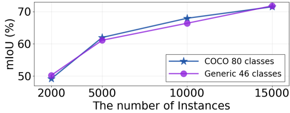
Figure 13: Comparison with different class sets for the auxiliary region extraction (Sec. 3.2 in the manuscript) on RefCOCO dataset for a RIS task. Each class set is prompted into Grounded-SAM to extract auxiliary regions. The generic 46-class set is shown in Tab. 8.
