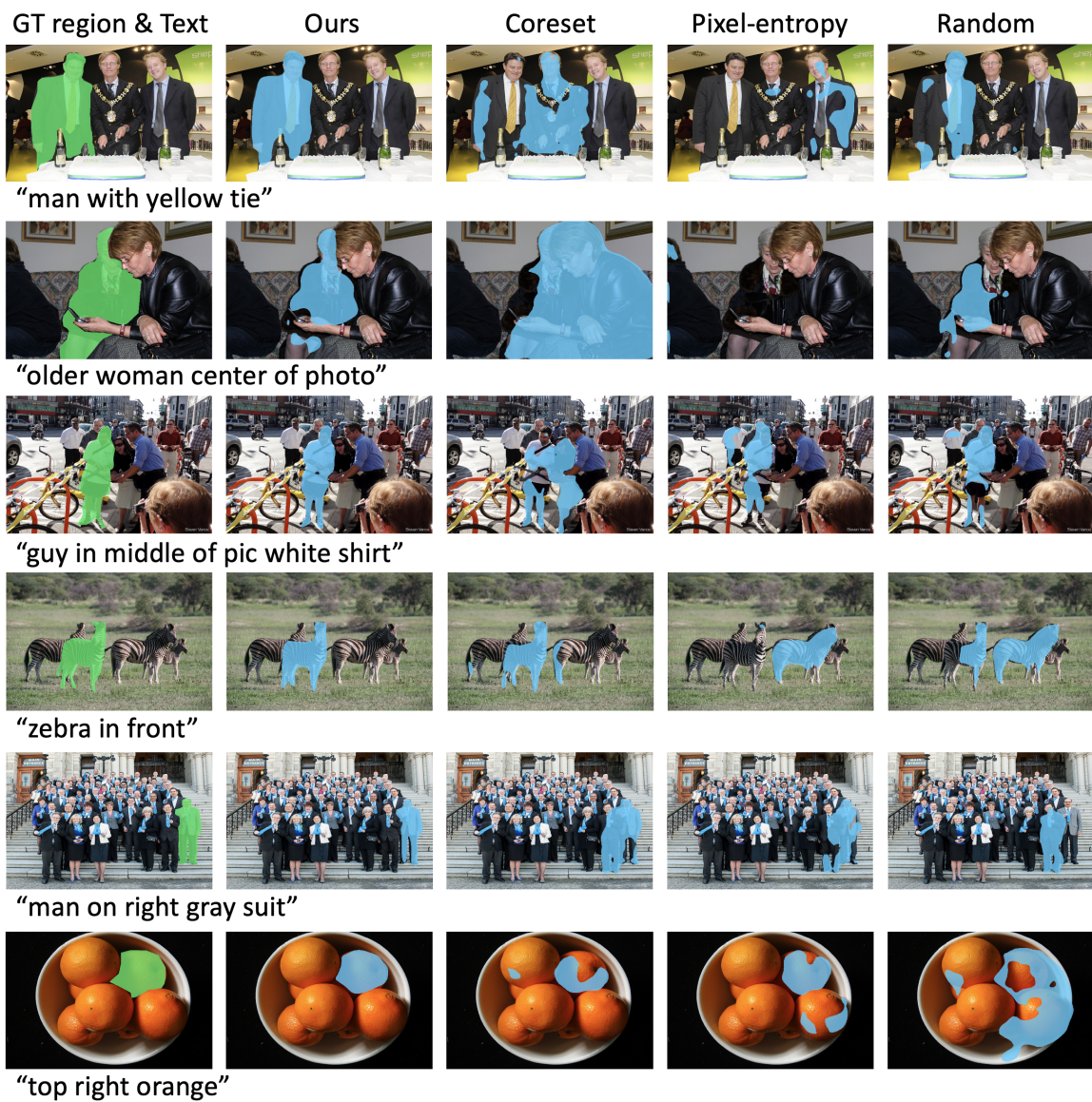
Figure 19: Qualitative examples from the ambiguous subset compared with the RIS models trained under different acquisition strategies.
