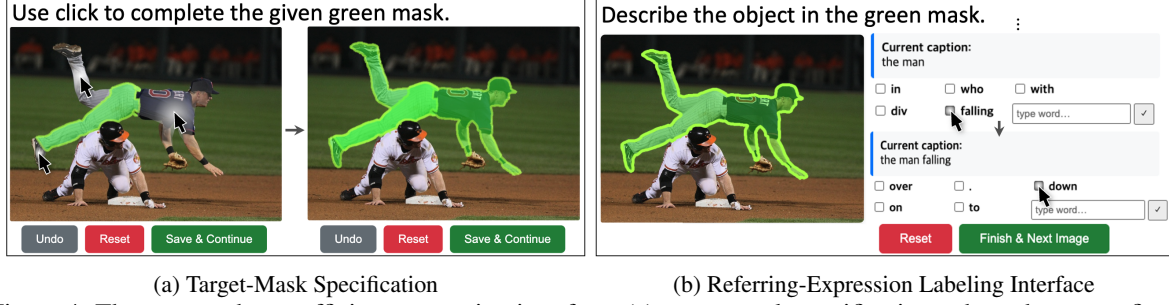
Figure 4: The proposed cost-efficient annotation interface. (a) target-mask specification, where the user refines a presented mask by clicking on a desired region in sequence, and (b) text labeling interface, where the annotator composes a referring expression for the green mask by clicking on suggested word candidates sequentially, with the option to manually type a word if none of the suggested words are suitable. Demo videos are available in our GitHub repository .
