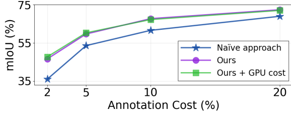
Figure 14: Comparisons under a fixed U.S. dollar budget that accounts for the GPU overhead in our approach. The cost estimates are summarized in Tab. 9.
