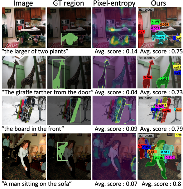
Figure 18: Additional qualitative analysis on the process of computing the informativeness score compared to the pixel-entropy.
