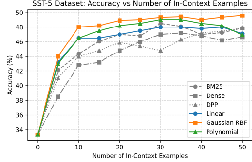
Figure 2: Accuracy comparison of the Qwen-1.5B model on the SST-5 dataset across varying numbers of in-context examples (ICE). The KITE algorithm, using kernel-based selection strategies, significantly outperforms baseline methods (BM25, Dense, DPP) in low-ICE settings.
