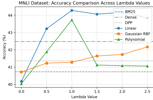
Figure 1: Ablation study on the MNLI dataset illustrating the effect of varying \lambda values. We report accuracy for KITE using different kernel-based selection strategies on the Qwen-1.5B model. Since MNLI has a large example bank (over 400k examples), a purely relevance-based selection ( \lambda = 0 ) underperforms. Incorporating diversity through higher \lambda values (e.g., \lambda = 1 ) leads to notable improvements in accuracy by promoting a more diverse selection of in-context examples.
