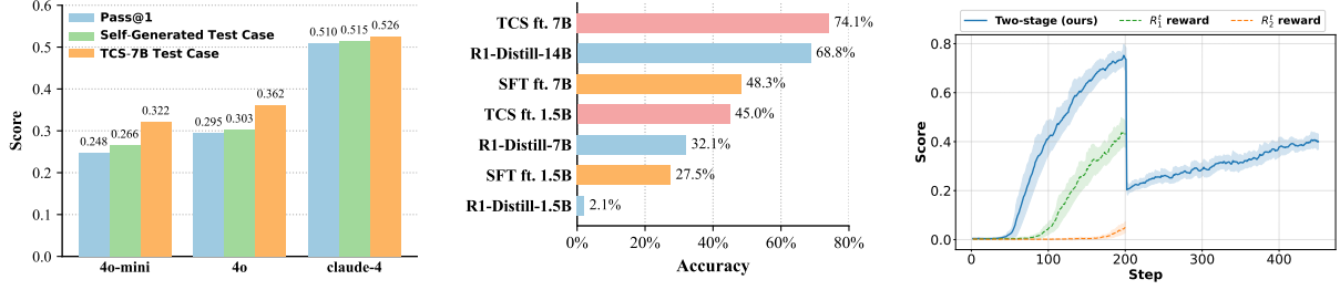
Figure 4: (a) Pass@1 (blue) and BoN ( N=8 ) (green/orange) performance selected by self-generated or TCS-7B-generated test cases for strong external models in LiveCodeBench. (b) Test case output prediction accuracy. The abbreviation “ft.” denotes finetuned models. (c) Scores under different training rewards.
