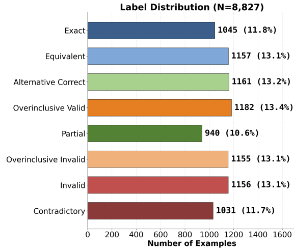
Figure 4: Distribution of semantic correctness labels in CAP-Correctness.
