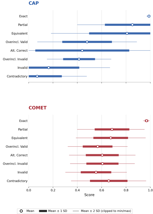
Figure 3: Geometric representation of CAP vs COMET.
