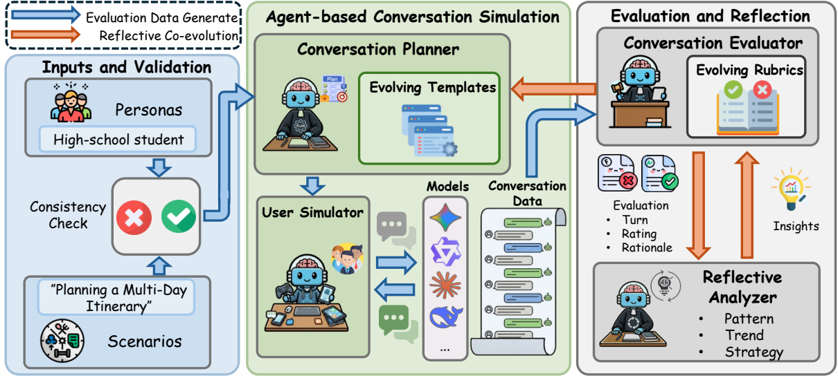
Figure 1: Overview of the CoReflect framework. Initially, evaluation instances are generated from persona-scenario pairs and validated through a consistency check to ensure contextual coherence. Then the core co-evolution loop proceeds through two parts: (i) Conversation simulation, where a planner generates structured conversation templates to guide a user simulator through goal-directed dialogues across diverse persona-scenario pairs; and (ii) Reflective rubric refinement, where an LLM-as-a-judge evaluates simulated interactions and a reflective analyzer extracts insights from clustered behavioral patterns to refine evaluation rubrics. The insights are fed back to the planner to update conversation templates for subsequent iterations.
