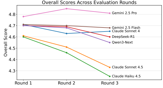
Figure 2: Model ratings across iterations. Iterative reflection improves model differentiation, yielding more distinct stratification and relative ordering.
