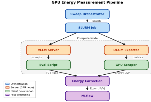
Figure 1: Scheme of the measurement
