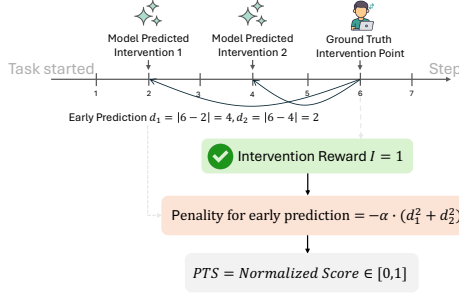
Figure 2: Visual illustration of how PTS is calculated. We measure the squared L_2 distance between the ground-truth intervention and false-positive predictions, and penalize the score based on that distance.
