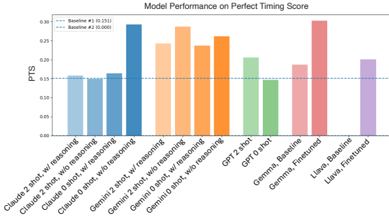
Figure 4: Perfect Timing Score on COWCORPUS. Among the proprietary models, Claude outperforms GPT-4o and Gemini-2.5, while fine-tuned Gemma 27B achieves the best overall result on COWCORPUS.
