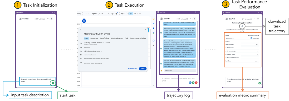
Figure 8: Overview of the collaborative AI agent, COWPILOT (Huq et al., 2025) used in our data collection. 1) Before the task is initiated, the user gives a textual task description as input. 2) During task execution, the system tracks the actions performed by the user and the agent. 3) After the task is executed, the user can download the task log.
