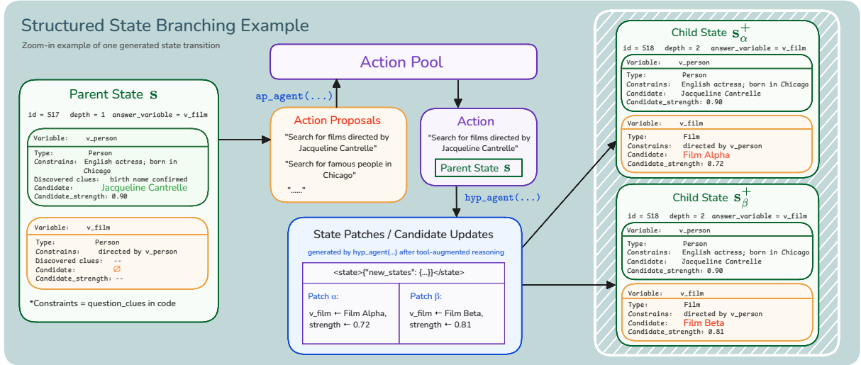
Figure 3: Structured state transition example. A partially resolved parent state grounds an action proposal, whose execution emits candidate updates for the unresolved answer variable. Applying these updates creates parallel child states that inherit shared assignments while branching over alternative candidates.
