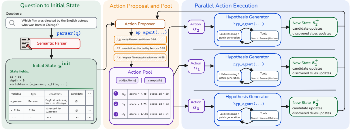
Figure 2: Overview of Gnosis Deepsearch
