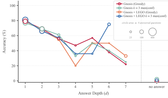
Figure 5: Performance of Gnosis variants with gpt-oss-20b at different answer depths across different retrieval and answer selection strategies. The circle area in each graph is proportional to the number of questions answered at that depth.
