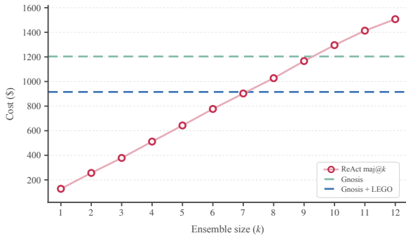
Figure 6: Analysis of how Gnosis’s test-time compute budget is matched across different numbers of ReAct trajectories, with k \leq 12 .
