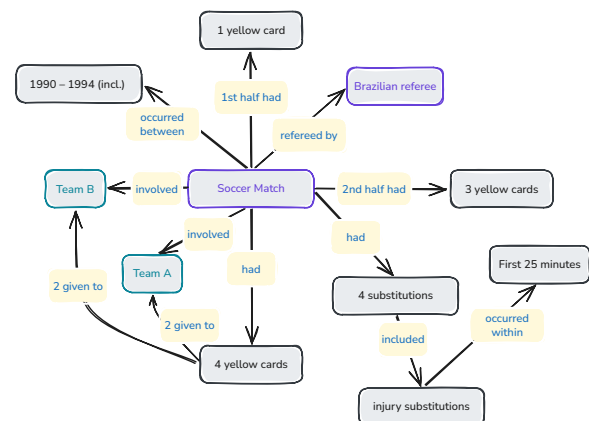
Figure 1: The graph corresponding to a complex question from BrowseComp-Plus: “Between 1990 and 1994 (inclusive), what teams played in a soccer match that had a Brazilian referee, included four yellow cards – two for each team – where three of the total four were not issued during the first half four substitutions, one of which was for an injury during the first 25 minutes of the match?”.
