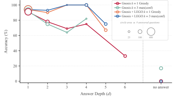
Figure 4: Performance of Gnosis variants with DeepSeek-V4-Flash at different answer depths across different retrieval and answer selection strategies. The circle area in each graph is proportional to the number of questions answered at that depth.
