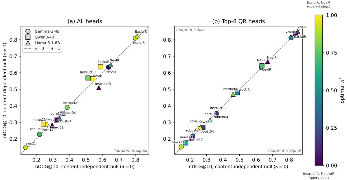
Figure 4: \lambda=0 vs. \lambda=1 nDCG@10 under pre-document placement (instruction before the documents, outside the readout); cf. Fig. 2 (readout placement). With the instruction out of the readout its null-pass footprint nearly vanishes, so calibration neither helps nor hurts: nearly all points lie on the diagonal and the InstructIR catastrophe disappears.
