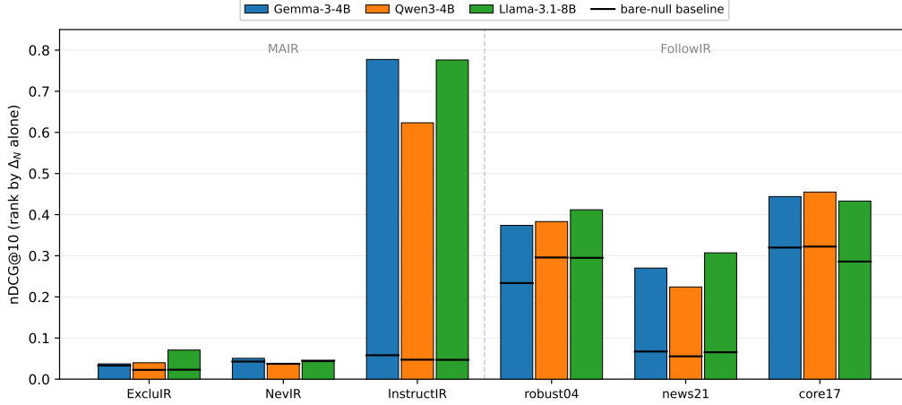
Figure 3: Ranking documents by the instruction’s null-pass effect \Delta_N alone (query replaced by “N/A,” documents in random order so position is decorrelated from relevance), nDCG@10, for three models. Black ticks mark the bare-null baseline (ranking by s_d(\emptyset, \emptyset) alone). \Delta_N alone ranks InstructIR documents far above its near-zero baseline but carries essentially no relevance signal for the shared-instruction tasks ExcluIR/NevIR. This is direct evidence that the null pass holds content- dependent relevance signal only for per-query instructions.
