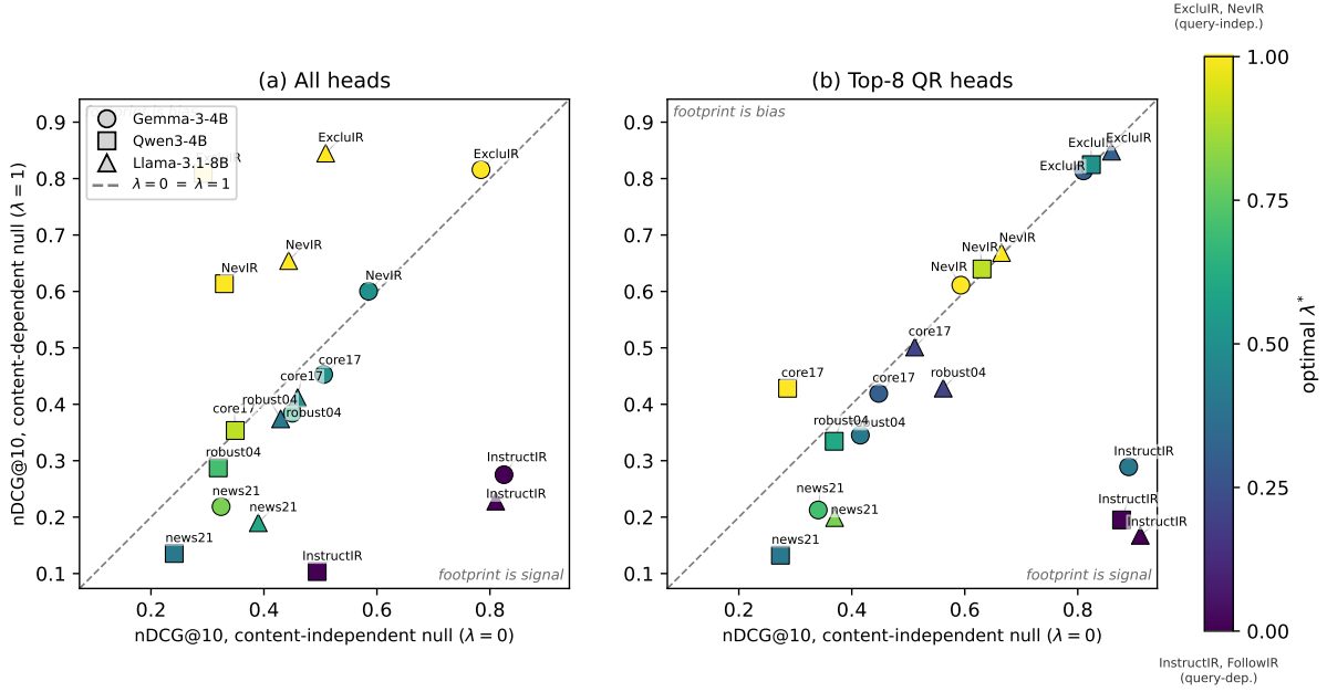
Figure 2: Comparison of reranking performance under the bare null ( \lambda=0 , x -axis) versus the instruction-inclusive null ( \lambda=1 , y -axis) for every (model, task). Marker shapes denote the model, and colors indicate the optimal interpolation parameter \lambda^* . Panel (a) evaluates all attention heads, while panel (b) isolates the top-8 query-relevance heads. Regions above the diagonal represent tasks benefiting from standard calibration, while regions below indicate tasks where instructions provide relevance signal, which subtraction destroys.
