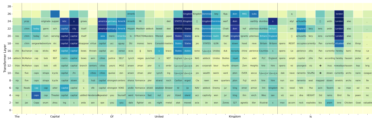
Figure 17: Logit Lens of inner states of the spoken input: "The capital of United Kingdom is...", using Llama-3.2 PI-1/3 (official). This version contains less filters on the time and layer domain and thus show higher resolution in the inner mechanism by logit lens perspective
