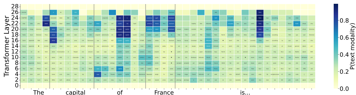
Figure 23: Logit Lens of inner states of the spoken input: "The capital of France is...", using Llama-3.2 PI-1/3 (official).
