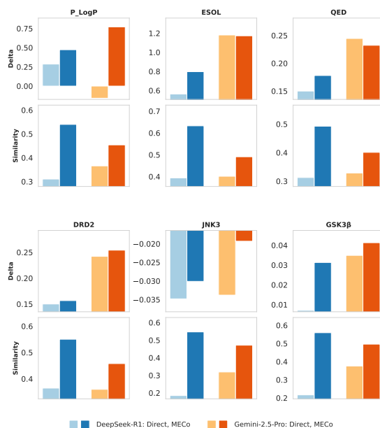
Figure 9: Bar plots of molecular optimization performance across six tasks, showing property improvement (top row) and structural similarity (bottom row) for Direct generation and MECo for DeepSeek-R1 and Gemini-2.5-Pro.
