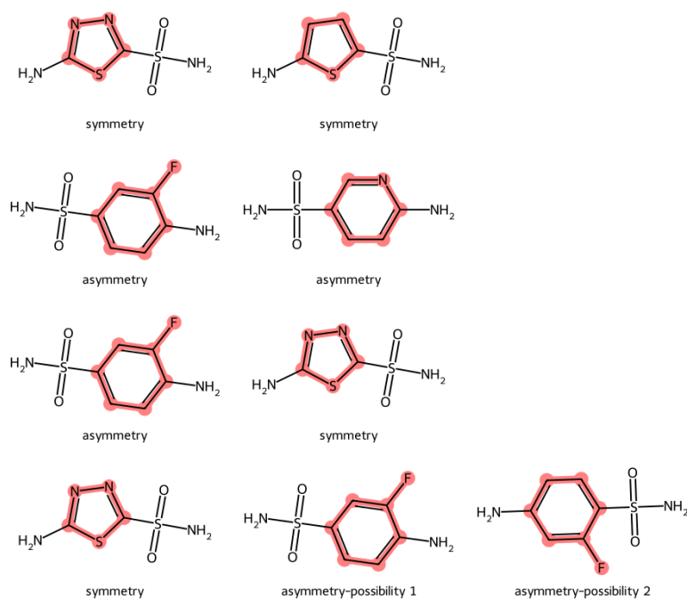
Figure 5: Multiple possible permutations in symmetry-to-asymmetry core replacement.
