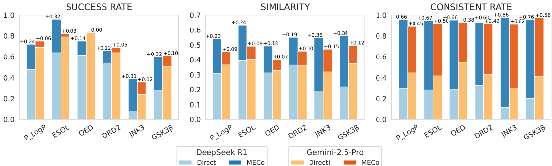
Figure 3: Incremental bar plots comparing direct generation (light bars) and MECo (dark stacked bars) across tasks and metrics under two different reasoning LLMs. Numbers above the bars indicate the absolute improvements of MECo over direct.
