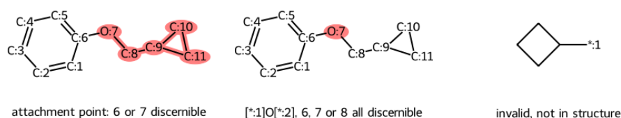
Figure 8: Visualization of manual check criteria.
