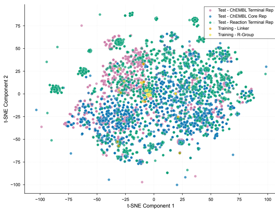
Figure 6: t-SNE for fragments in synthetic training data construction and realistic edit test set.
