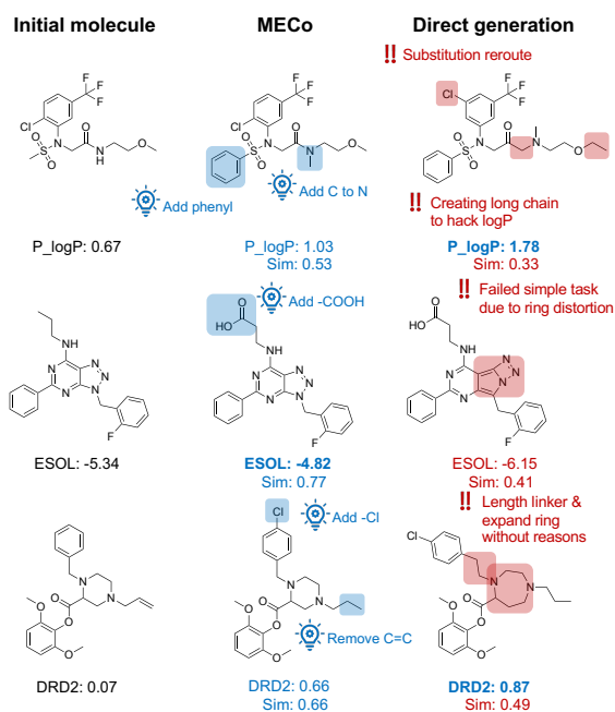
Figure 4: Representative case study of molecular modification. (A) Direct generation produces uncontrolled changes and low similarity, often leading to unrealistic score inflation or failed optimization; MECo achieves improved scores and higher similarity through interpretable, chemistry-preserving edits. (B) MECo demonstrates coherent consistency across the reasoning–execution–analysis pipeline.
