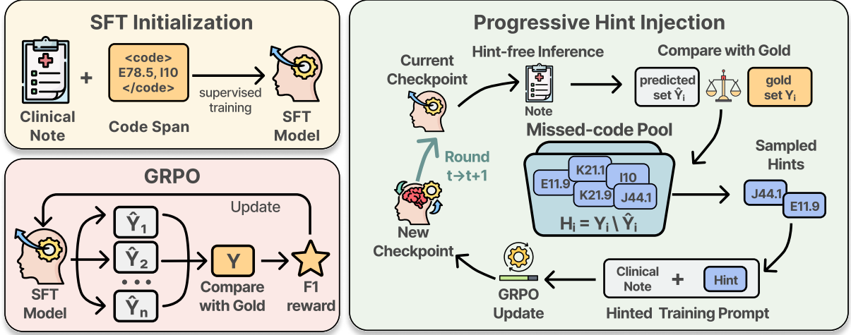
Figure 2: Overview of our post-training pipeline. A generative large language model (LLM) is first adapted through supervised fine-tuning (SFT) to emit a parseable code span. Vanilla Group Relative Policy Optimization (GRPO) and Progressive Hint Injection (PHI) are then initialized independently from the same SFT checkpoint. GRPO optimizes sample-level code-set F1 over the full training set, whereas PHI iteratively performs hint-free inference, collects missed codes Y_i \setminus \hat{Y}_i into per-sample pools, and samples training-time hints for the next adaptive round. Hints are used only during training; inference remains hint-free.
