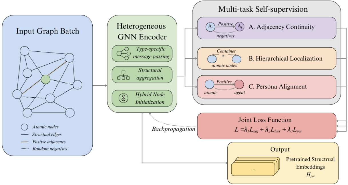
Figure 3: Stage 1: Multi-Task Structural Pre-training. Before accessing motif labels, the encoder is forced to internalize the narrative “anatomy” via three intrinsic objectives: (A) Adjacency Continuity ( u_t \rightarrow u_{t+1} ) captures local discourse flow; (B) Hierarchical Localization ( u \rightarrow s ) recovers macro-structural positioning; and (C) Persona Alignment ( u \rightarrow a ) learns character-specific stylistic features. This structure-first strategy aligns the embedding space with the narrative topology.
