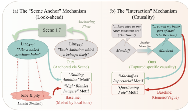
Figure 6: Structural reasoning beyond local cues. (a) CRITIC’S EYE anchors a metaphor to its scene context, avoiding a lexical-similarity trap. (b) CRITIC’S EYE propagates cross-speaker causality via interaction structure, resolving a specific motif where a sequential baseline predicts a generic one.
