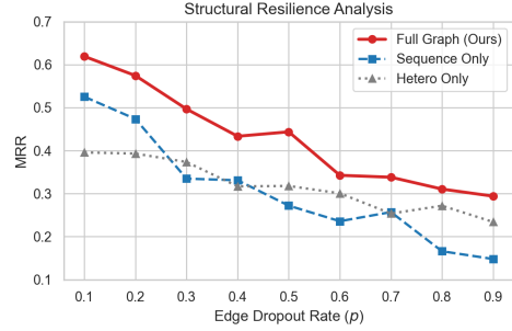
Figure 5: Structural resilience under edge dropout. Mean Reciprocal Rank (MRR) as a function of inference-time edge dropout rate p . The Full topology degrades more gracefully than Sequence-only across a wide range of dropout rates, indicating higher robustness to partial graph observations.
