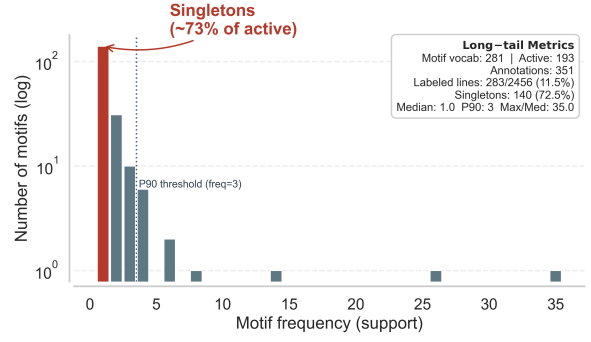
Figure 4: The Severe Long-Tail Distribution of Literary Motifs. MOTIFBENCH follows a sharp power law (Imbalance Ratio = 35.0), with over 96% of active motifs (187/193) in the sparse “tail” (freq \leq 5 ). This extreme sparsity renders standard random splits ineffective, motivating our transductive formulation to capture these rare signals.
