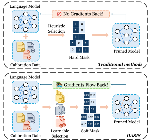
Figure 1: Traditional vs. OASIS . Traditional pruning blocks gradients, while OASIS enables feedback via soft masks and learnable calibration importance.
