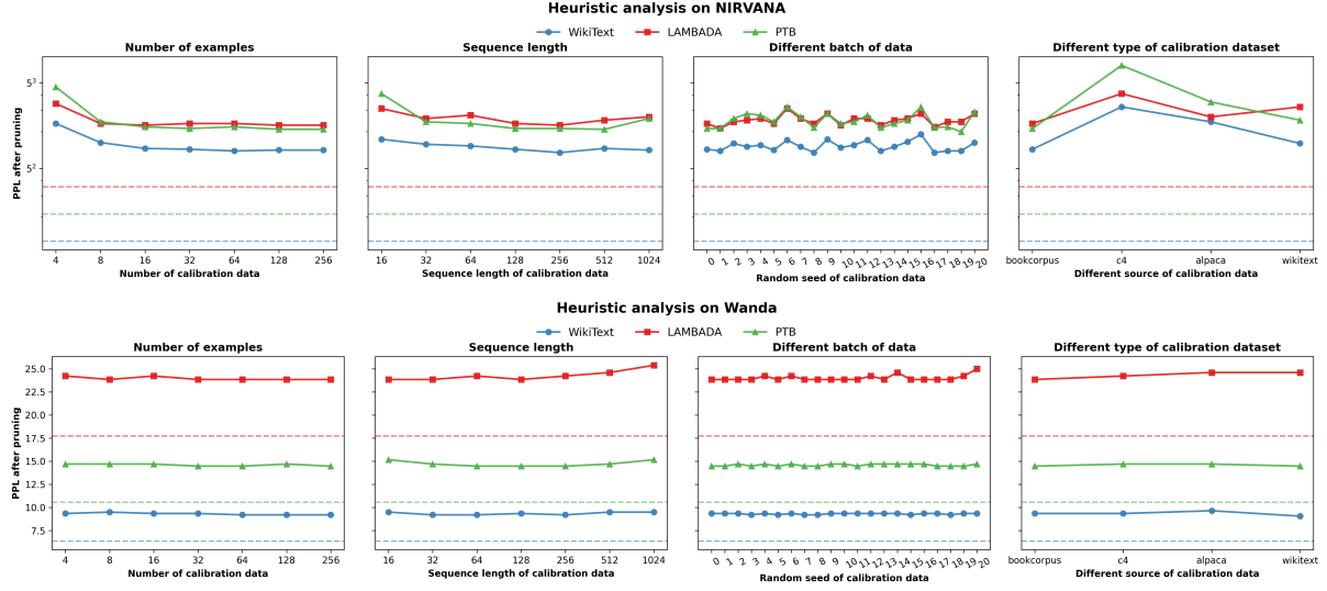
Figure 2: Macro-level analysis of how different heuristic choices for calibration data selection impact pruning performance. The top and bottom rows show results for the structured pruner (NIRVANA) and the unstructured pruner (Wanda), respectively. Each column investigates a different variable: (from left to right) the number of samples, sequence length, the random data batch, and the data source. The y-axis represents the post-pruning perplexity on three evaluation datasets: WikiText, PTB, and Lambada, indicated by separate colored lines. Dashed lines show the baseline perplexity of the unpruned model for comparison.
