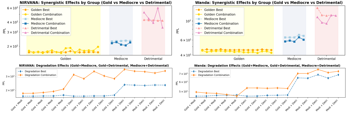
Figure 3: Micro-level analysis of calibration data interactions in NIRVANA (left) and Wanda (right). The top row investigates intra-tier synergy, comparing the performance of combining two samples from the same quality tier (e.g., "Golden Combination") against the performance of the better of the two individual samples ("Golden Best"). The bottom row demonstrates inter-tier degradation, showing the performance of combining samples from different tiers (e.g., "Golden + Detrimental") compared to the performance of the higher-quality sample in the pair ("Degradation Best").
