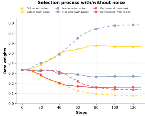
Figure 5: Evolution of importance weights during optimization. The dashed line (w/o noise) indicates overfitting to mediocre samples, while the full line (w/ noise) enables stable discovery of golden samples.
