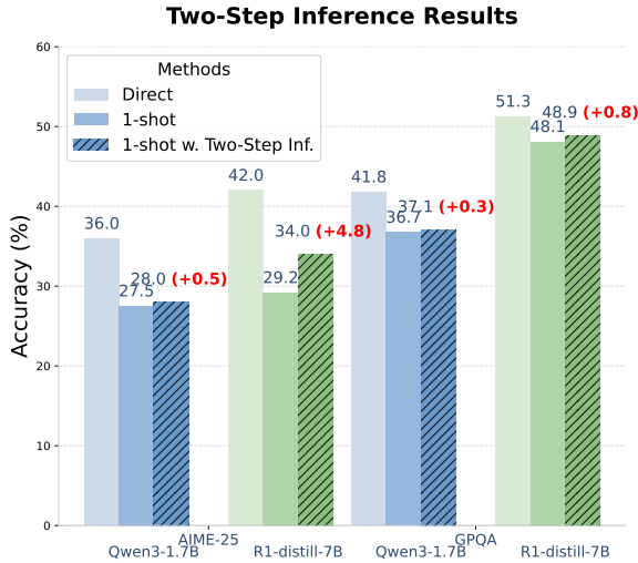
Figure 3: Results of two-step inference on AIME'25 and GPQA. Blue: Qwen3-1.7B; green: R1-Distill-Qwen-7B.
