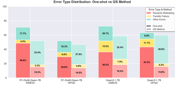
Figure 6: Failure-mode breakdown of one-shot in-context reasoning vs. I2S.
