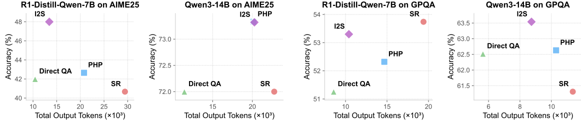
Figure 5: Generated-token cost versus accuracy. The full-width layout enlarges labels and separates model–dataset panels for readability.
