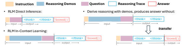
Figure 4: Three prompting paradigms. For Two-step inference (right), the demos are used only to elicit a trace; the demos are then removed and the final answer is generated from the question plus the elicited trace, decoupling answer generation from demo content.
