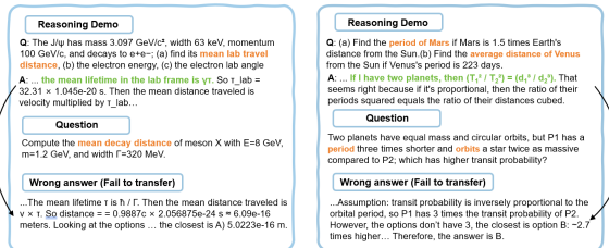
Figure 9: Failure modes in semantic misleading from demonstration content. (green: missed transferable insight).
