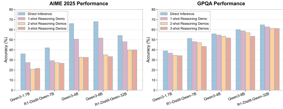
Figure 1: Few-shot CoT harms the RLMs performance, even with high-quality reasoning demonstrations.
