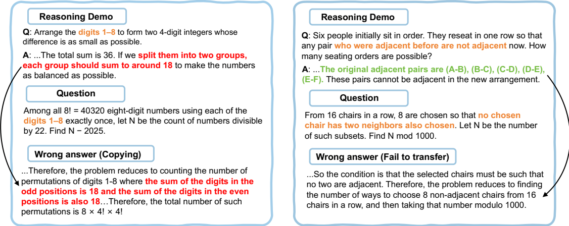
Figure 2: Failure modes in in-context reasoning. Left: Semantic misleading (red: inappropriate copying). Right: Failed structural transfer (green: missed transferable insight).
