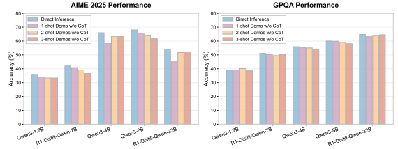
Figure 7: In-context learning with demonstrations that omit explicit thinking steps also harms the performance of reasoning language models (RLMs).
