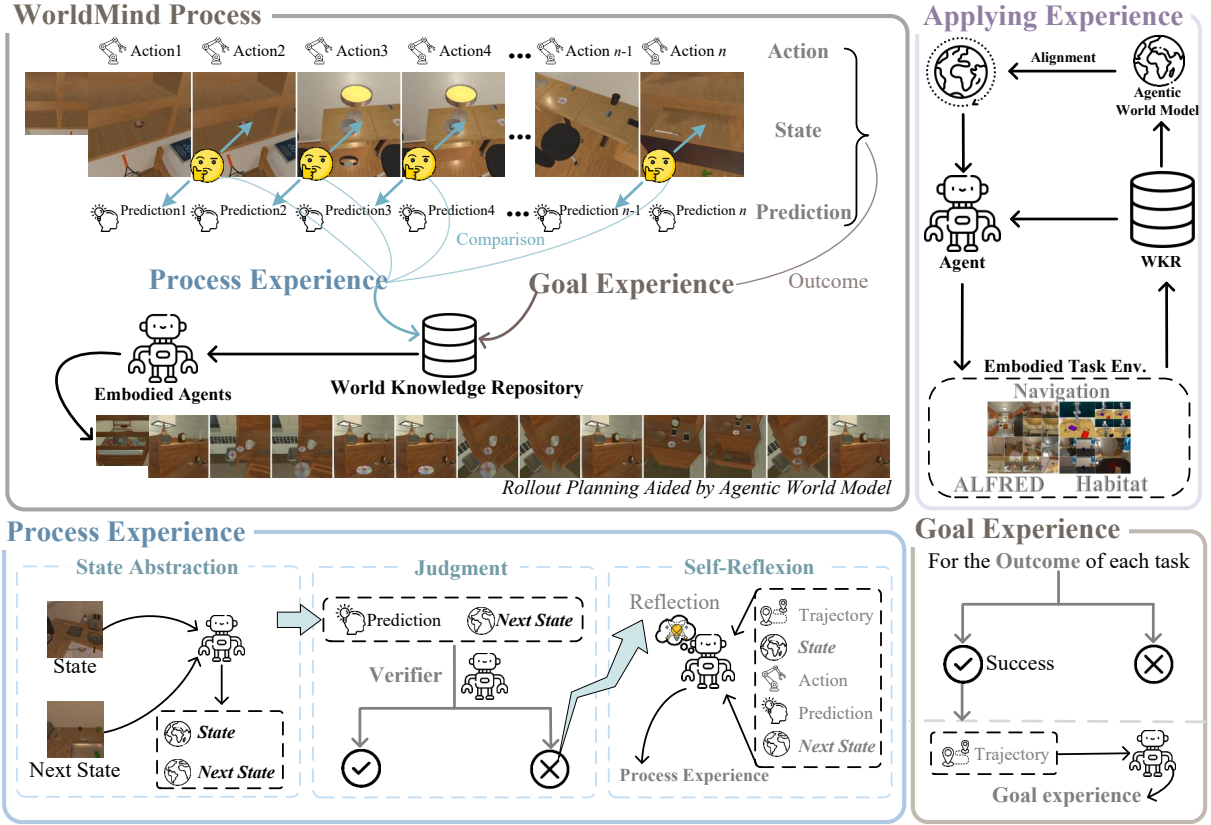
Figure 2: Overview of the WorldMind Framework. The agent autonomously constructs a World Knowledge Repository (WKR) by unifying Process Experience (from prediction errors) and Goal Experience (from successful trajectories) to guide grounded simulation.
