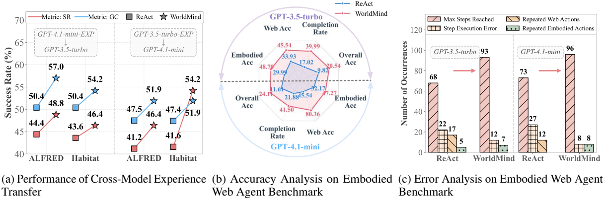
Figure 3: Experimental Results and Analysis. (a) Comparison of experience transfer capabilities between the two models. (b) Performance comparison on the Embodied Web Agent task, reporting accuracy metrics for both GPT-3.5-turbo and GPT-4.1-mini. (c) Comparative error distribution analysis for both models in the same environment.
