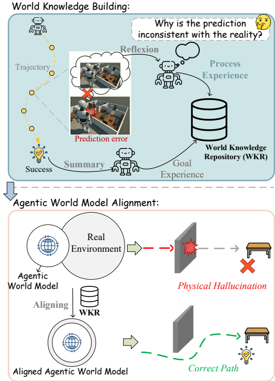
Figure 1: Conceptual Illustration of Experiential Alignment. The agent aligns its internal world model via Process Experience and Goal Experience.
