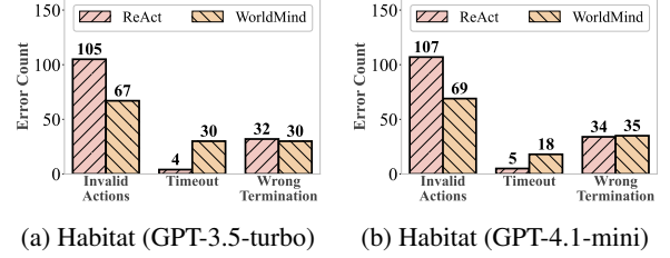
Figure 4: Error Analysis in EB-Habitat. Failure distributions for ReAct and WorldMind.
