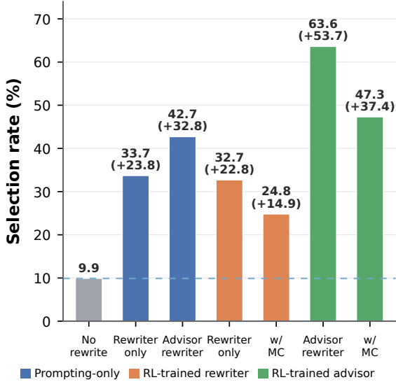
Figure 3: Selection rates on scientific-document impressions. MC: MiniCheck.
