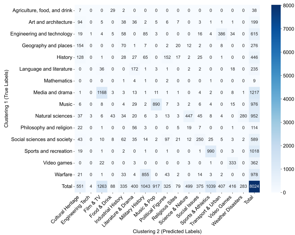
Figure 4: The contingency matrix of the ground-truth clustering and the best topical alignment experiment run of Textonomy.
