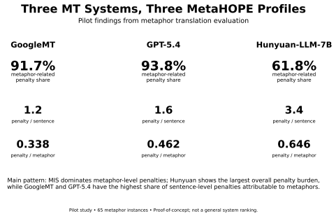
Figure 5: Three System Summary.
