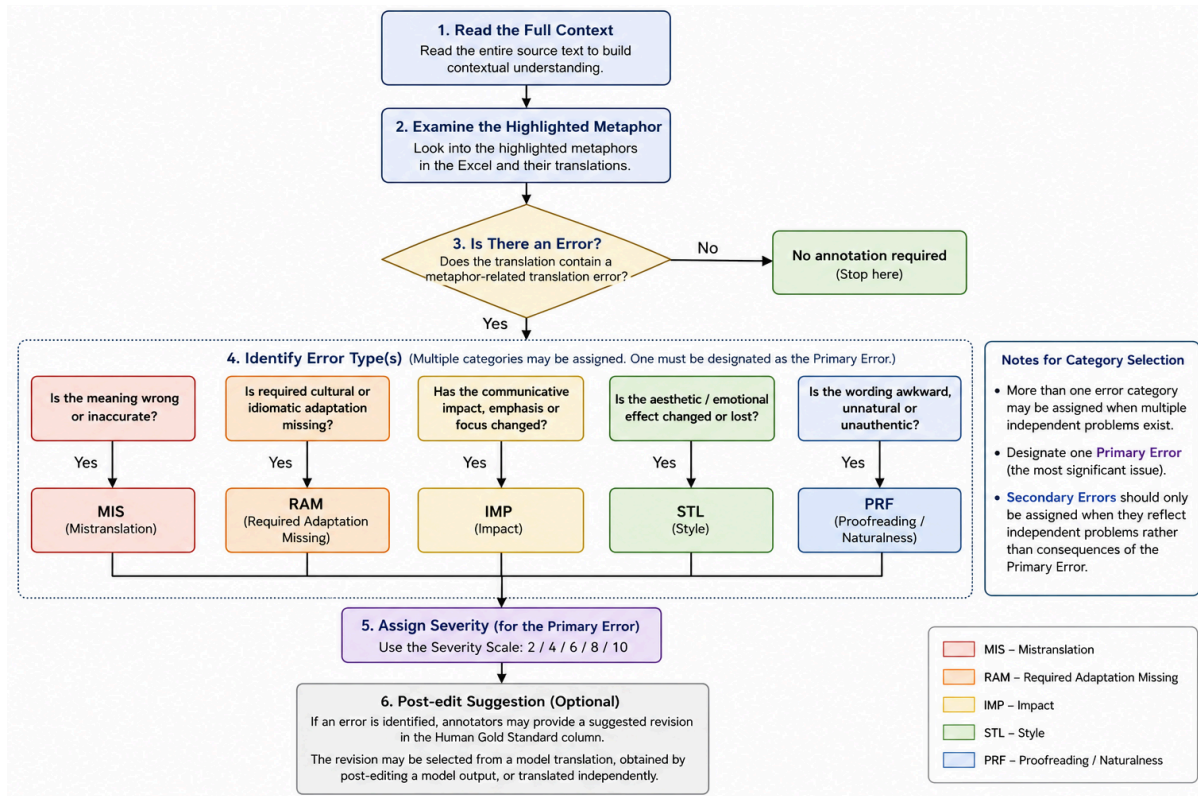
Figure 9: MetaHOPE Annotation Procedure via Decision Tree Illustration
