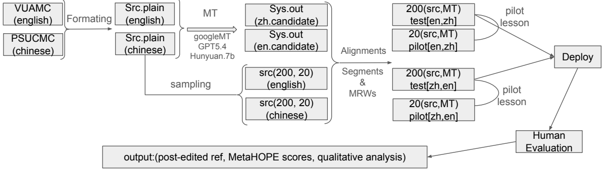
Figure 1: MetaHOPE Framework: Metaphor corpus preparation, MT, Aligning segments and metaphor-related words (MRWs), and post-editing with annotations on pilot (development) and test sets.
