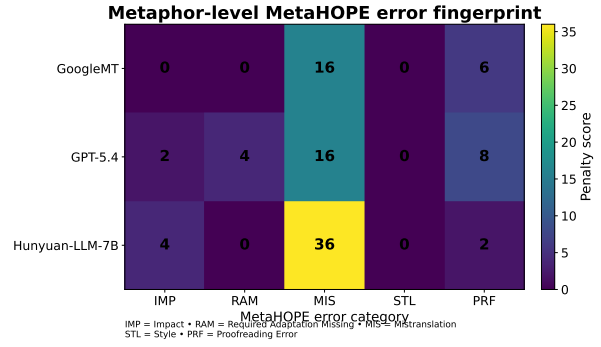
Figure 4: Error Type Heatmap.
