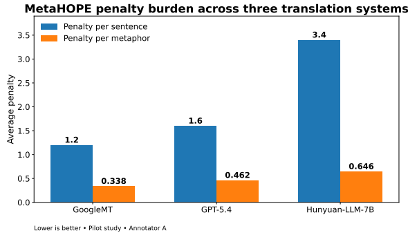
Figure 3: Penalty Comparison.
