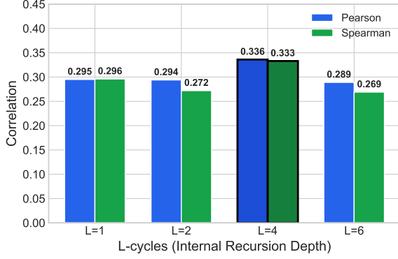
Figure 3: L-cycle ablation: performance peaks at L=4 (8 effective layers), with degradation at both shallower (L=1, L=2) and deeper (L=6) configurations.
