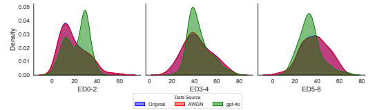
(a) GPT-4o - 2020
