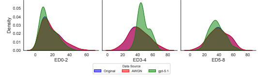
(c) GPT-5.1 - 2022
