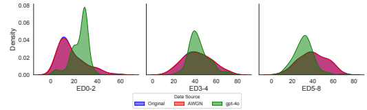
(c) GPT-4o - 2022
