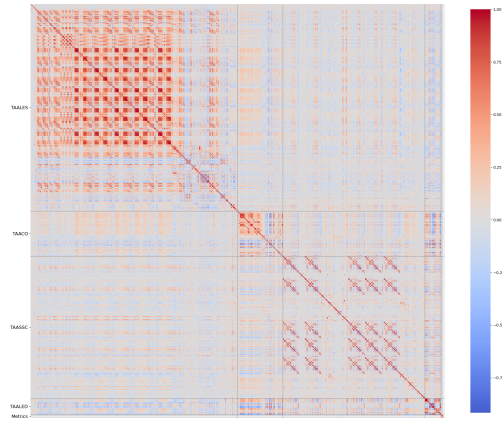
(b) Difference between original and simple, D-Wikipedia (document-level).
