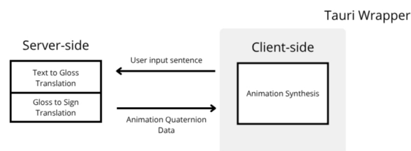
Figura 1. Architecture of the Synthesizer (Source: The Author)
