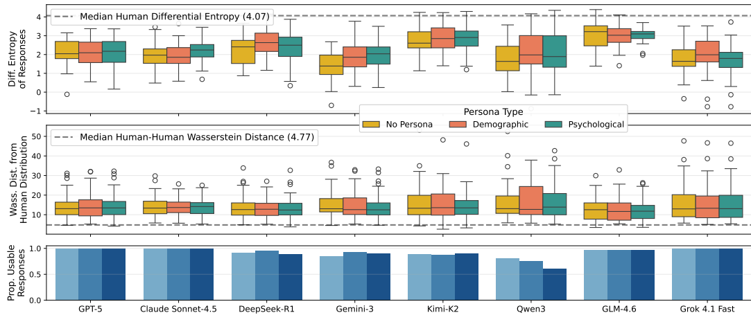
(c) Persona Prompting
