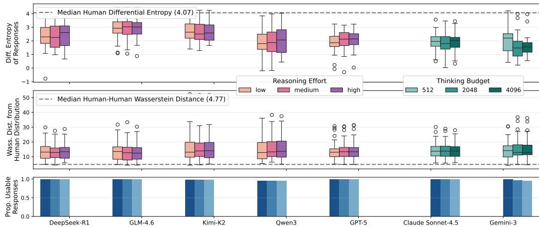
(b) Reasoning Effort
