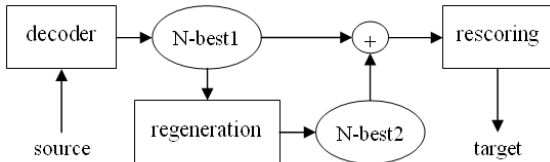
Figure 2: Structure of a three-pass machine translation system with the new regeneration pass. The original N-best translations list (N-best1) is expanded to generate a new N-best translations list (N-best2) before the rescoring pass.
